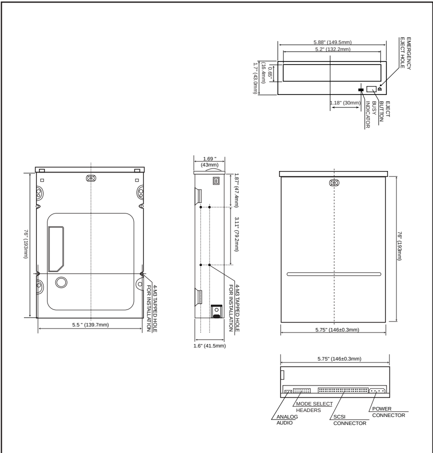
External Dimensions
